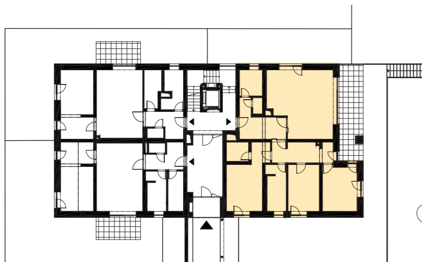
Location of the apartment on the floor
